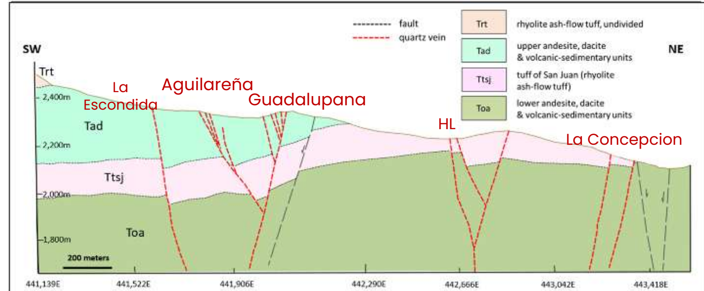
Generalized Cross-Section A – A', Aguilareña and Guadalupeana Area (from Durango Gold 2022, looking northwest)
